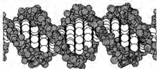
DNA molecule
